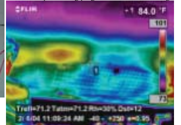
Infrared image of intra-laminate damages discovered preceeding plug confirmation of damages
